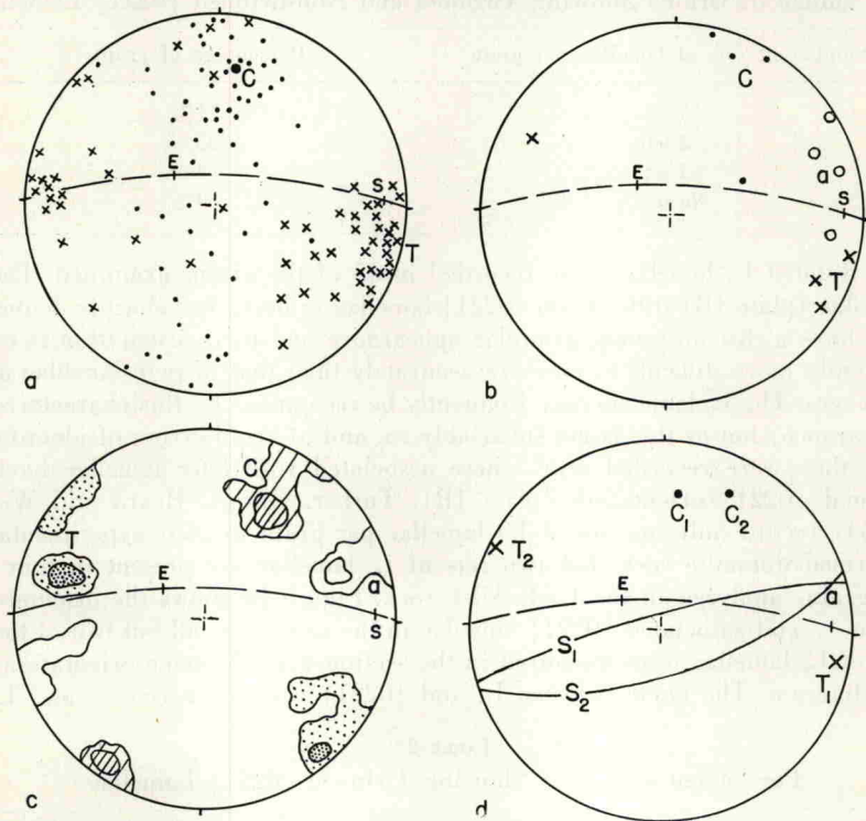
Fig. 3. Dynamic interpretation of data from the Loch Alish dolomite.
